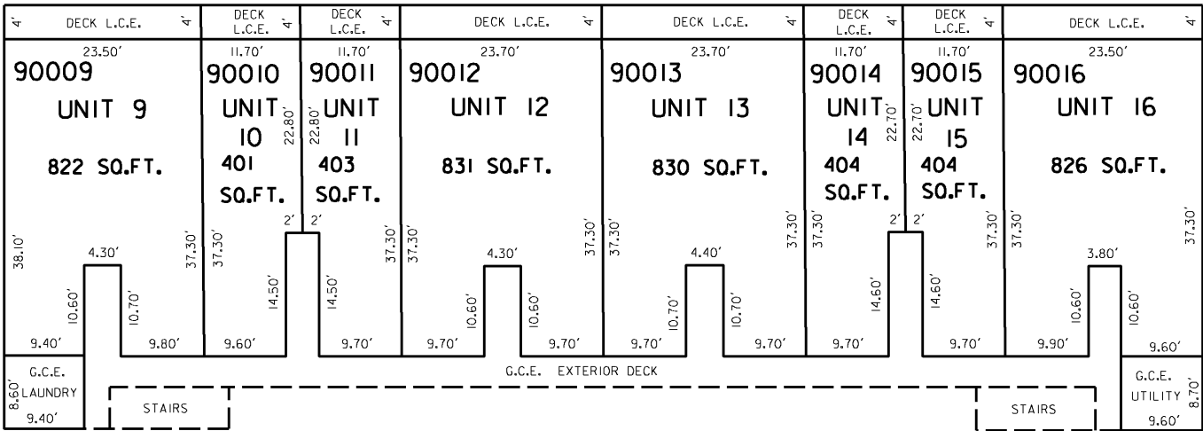
SECOND FLOOR
