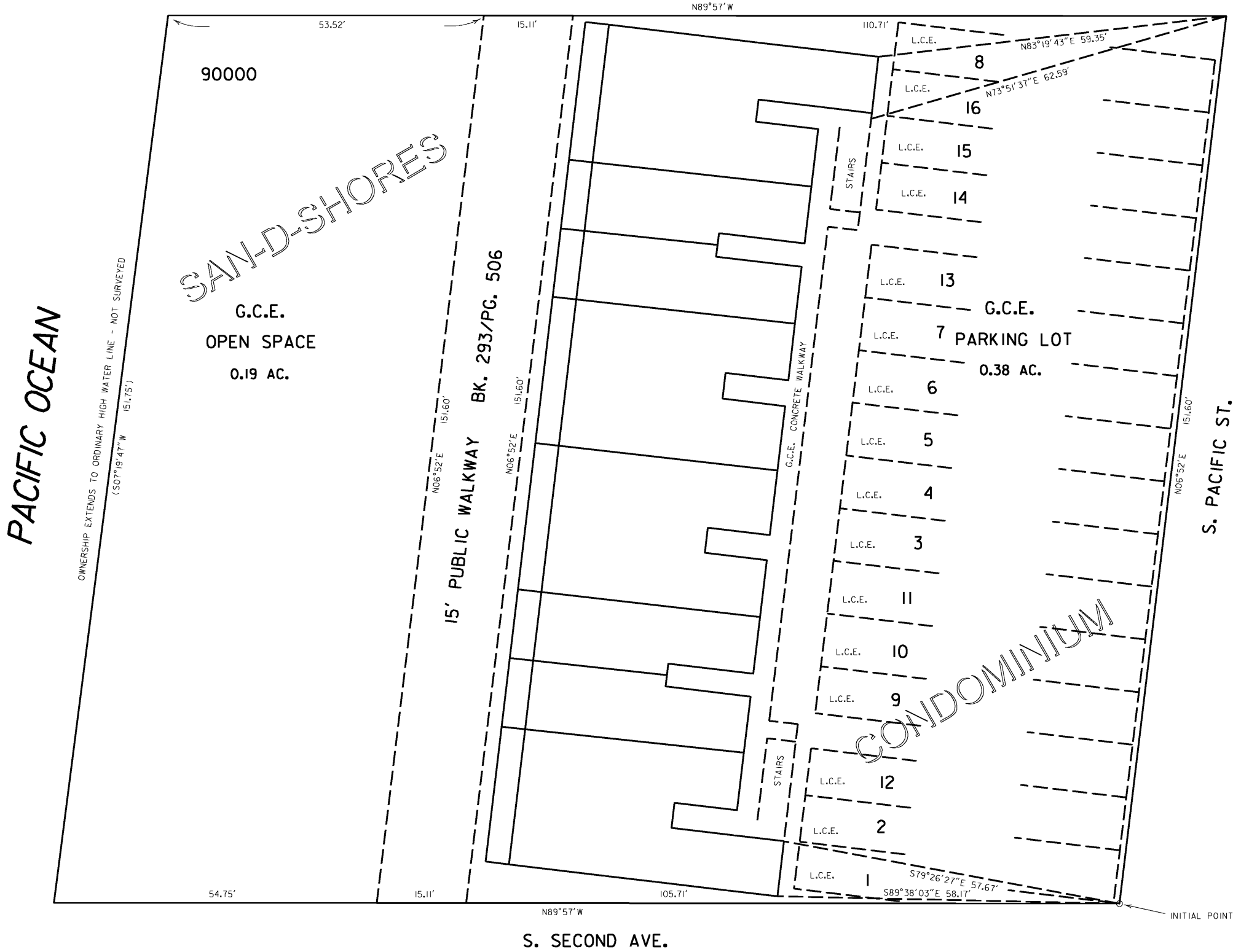
S. SECOND AVE. BUILDING LOCATION PLAN
